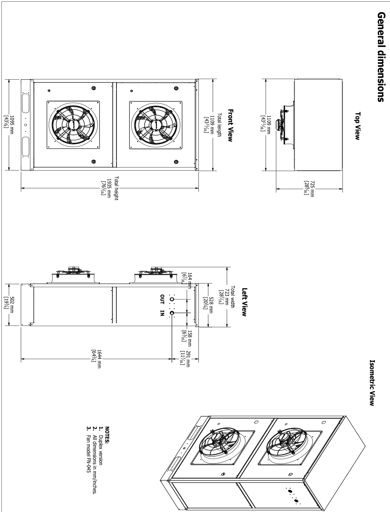
Figure 4. Dimensional configuration of the 10 RT unit.
