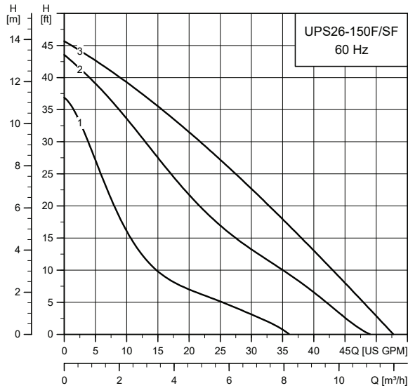
UPS 26-150 F/SF
