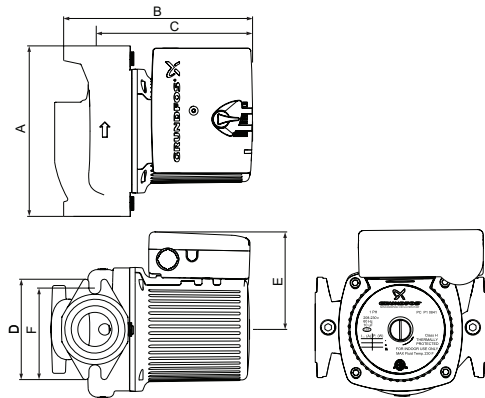
UPS 26-150 F/SF
